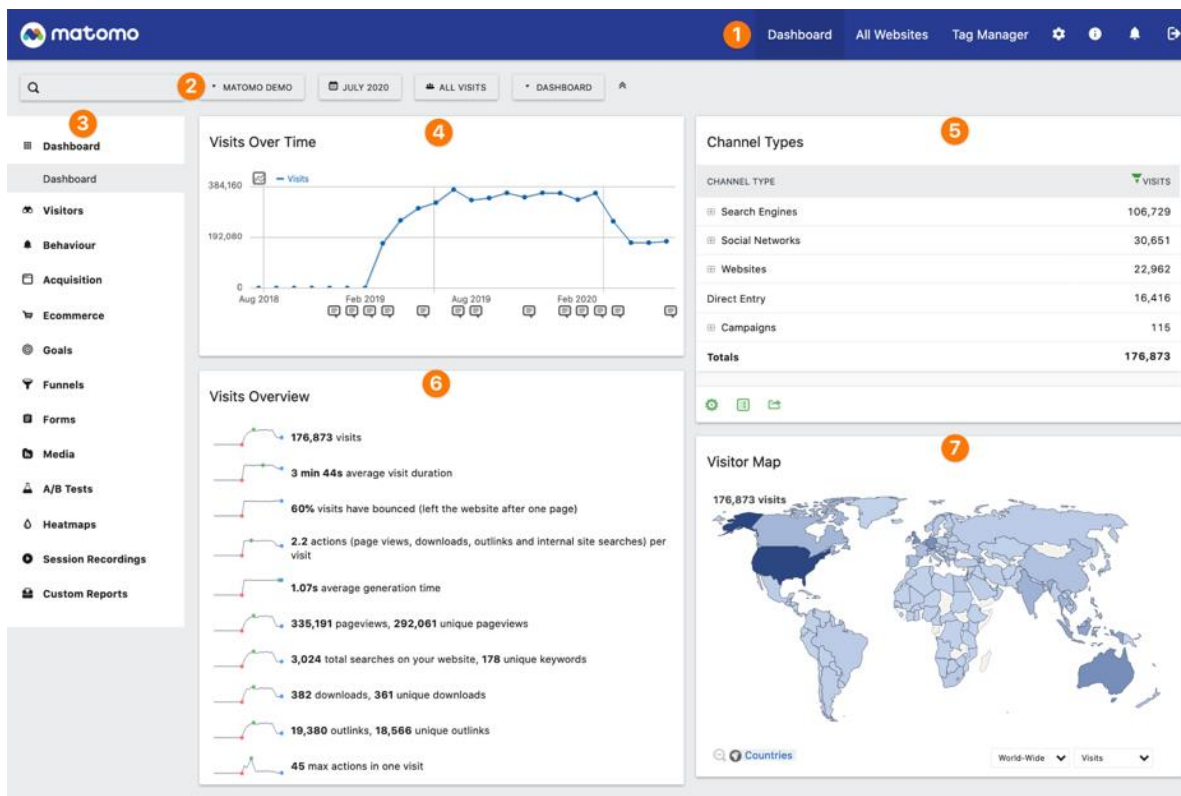
Figure 10: Matomo dashboard
